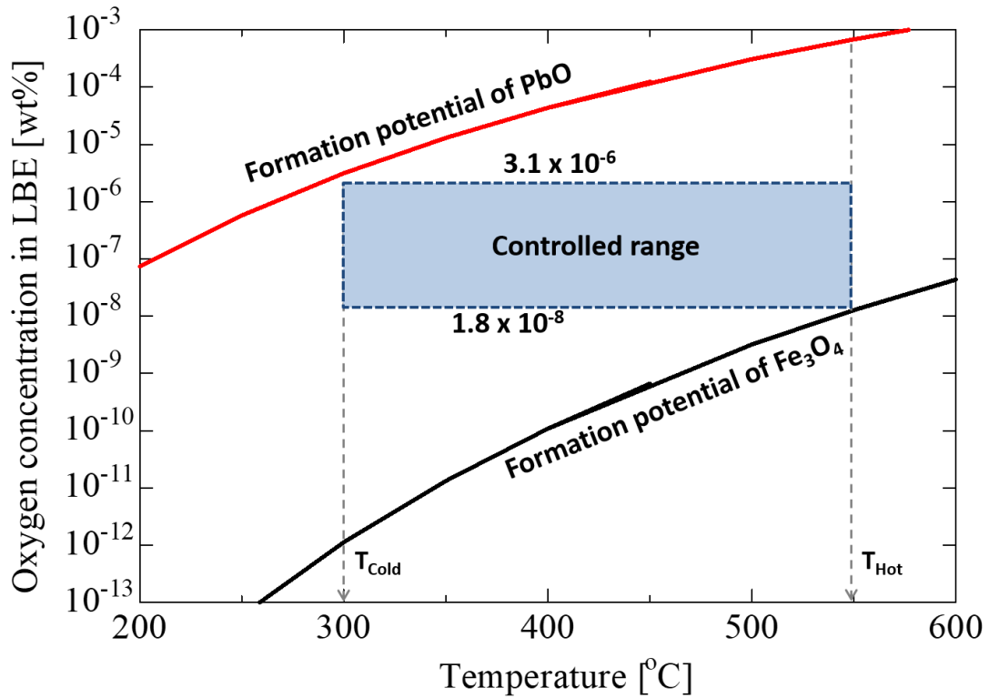
Figure 1. Oxygen control boundary of LBE cooled system
